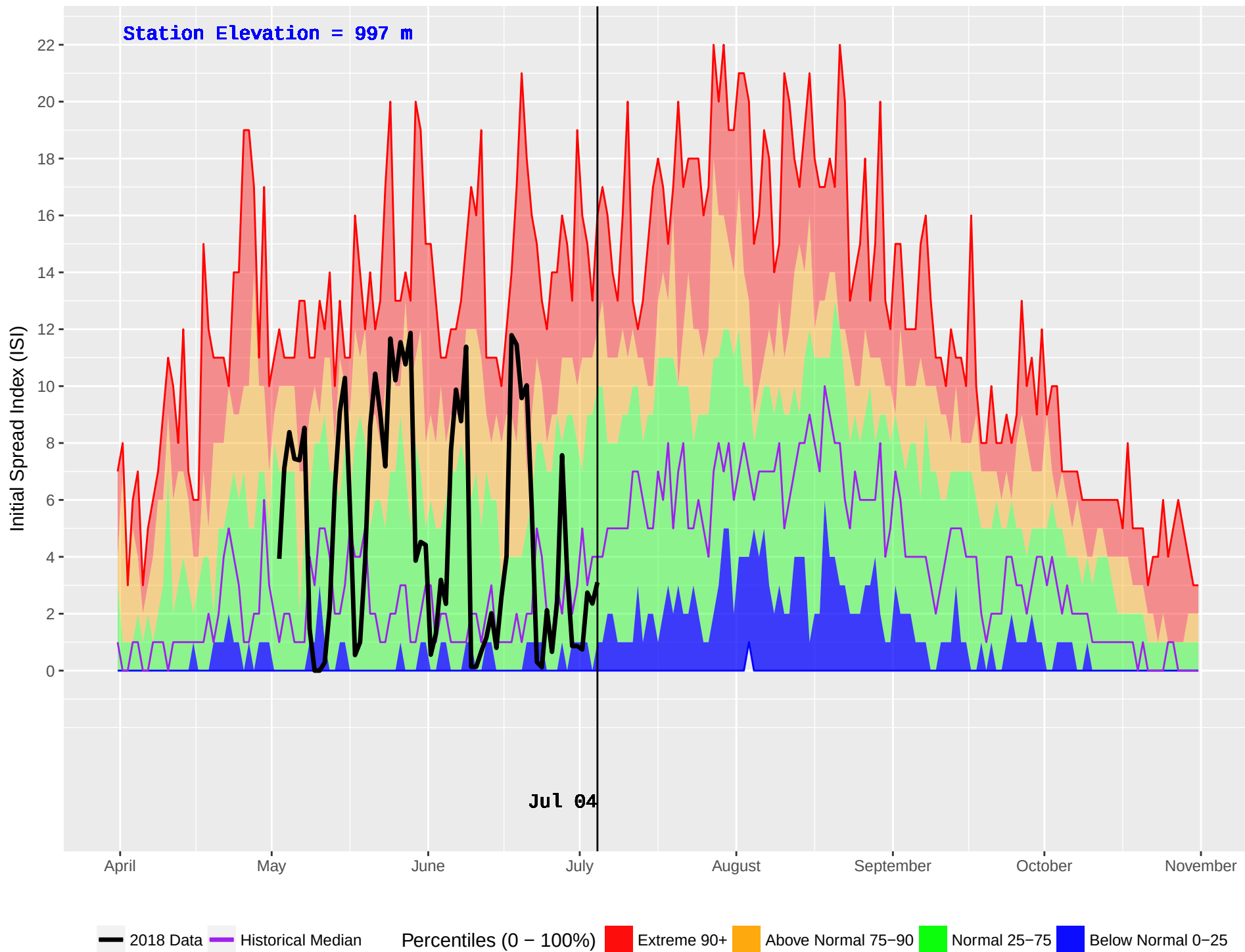
SMALLWOOD (404) : Historical (1991–2016) and Current (2018) Noon Initial Spread Index (ISI)
