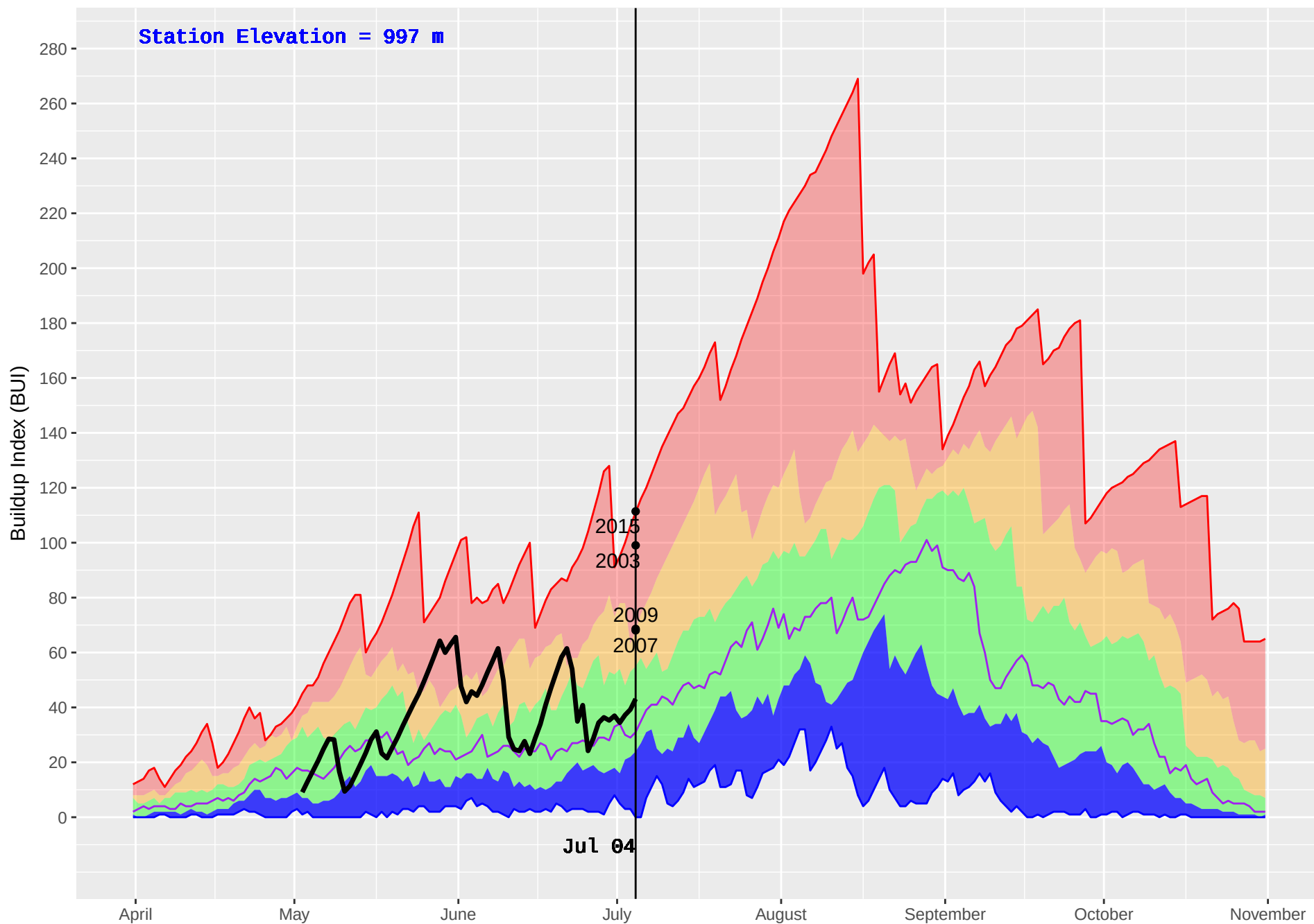
SMALLWOOD (404) : Historical (1991–2016) and Current (2018) Noon Buildup Index (BUI)
