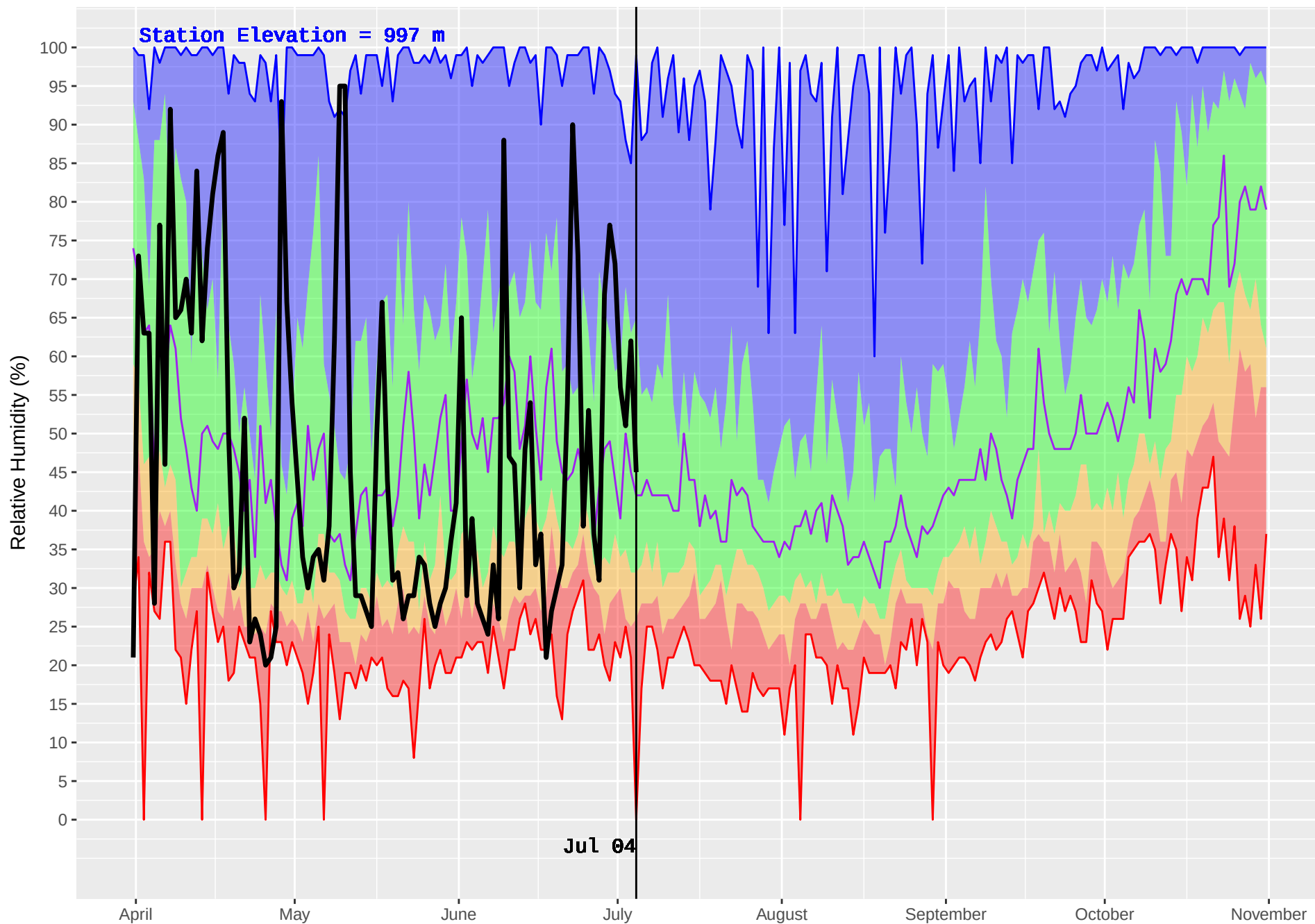
SMALLWOOD (404) : Historical (1991–2016) and Current (2018) Noon Relative Humidity
