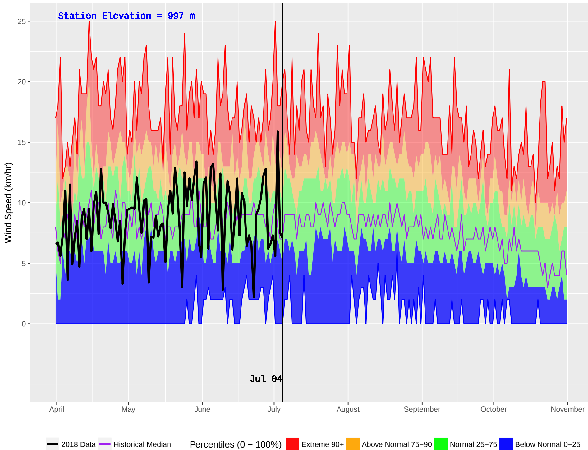
SMALLWOOD (404) : Historical (1991–2016) and Current (2018) Noon Wind Speed
