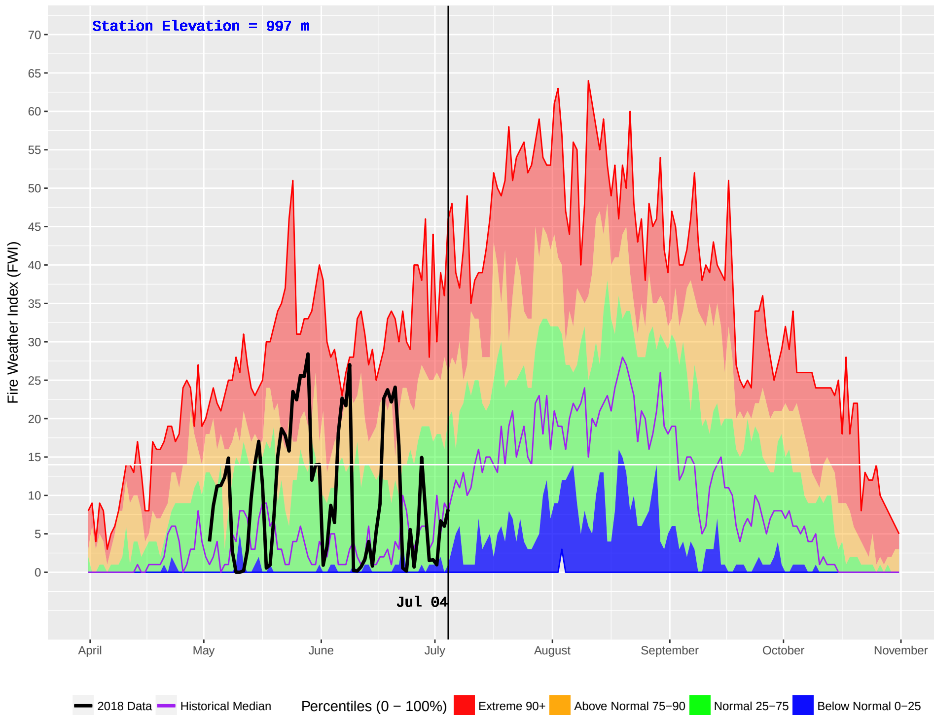
SMALLWOOD (404) : Historical (1991–2016) and Current (2018) Noon Fire Weather Index (FWI)
