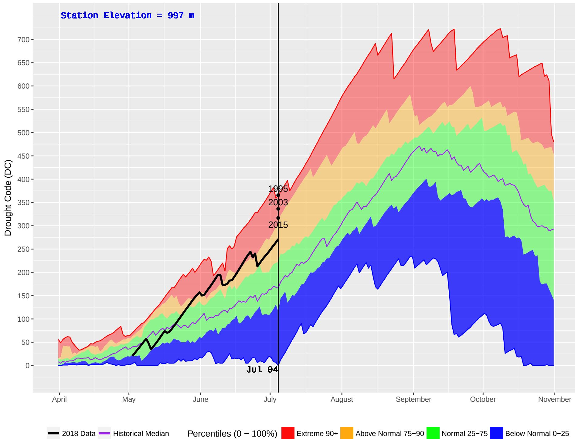
SMALLWOOD (404) : Historical (1991–2016) and Current (2018) Noon Drought Code (DC)
