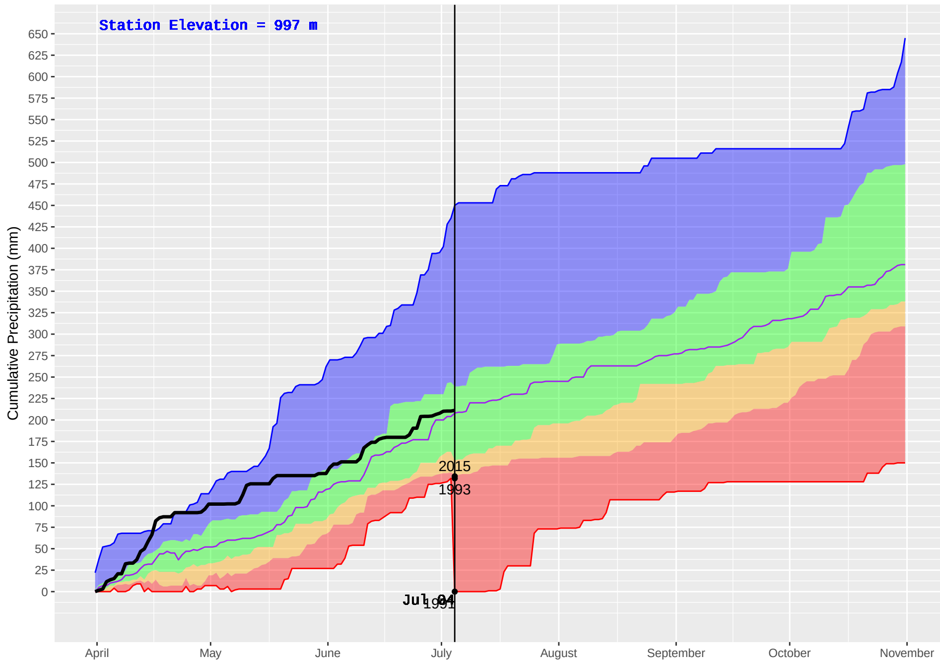
SMALLWOOD (404) : Historical (1991–2016) and Current (2018) Noon Cumulative Precipitation
