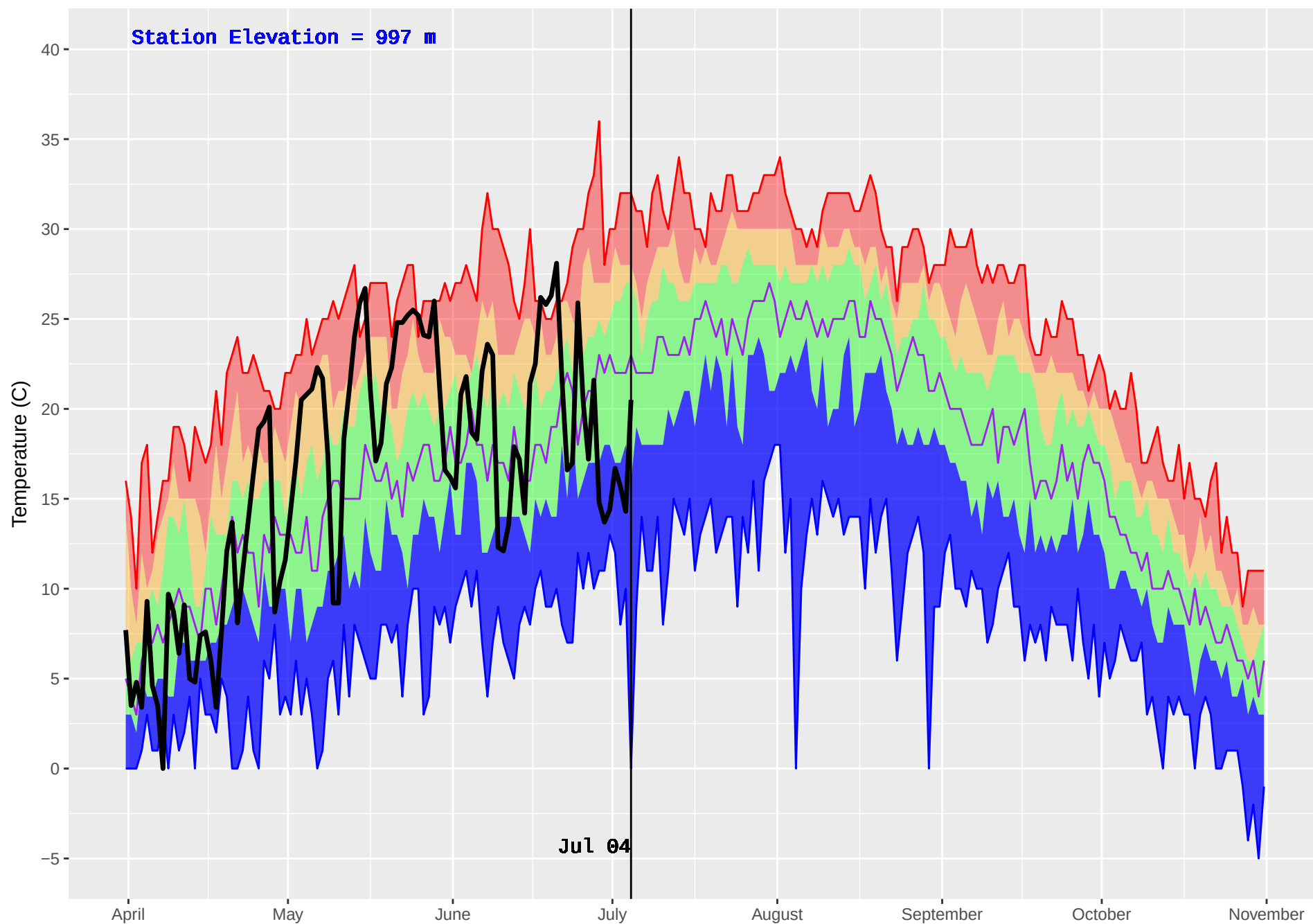
SMALLWOOD (404) : Historical (1991–2016) and Current (2018) Noon Temperature
